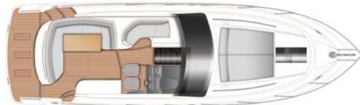
MAIN DECK
